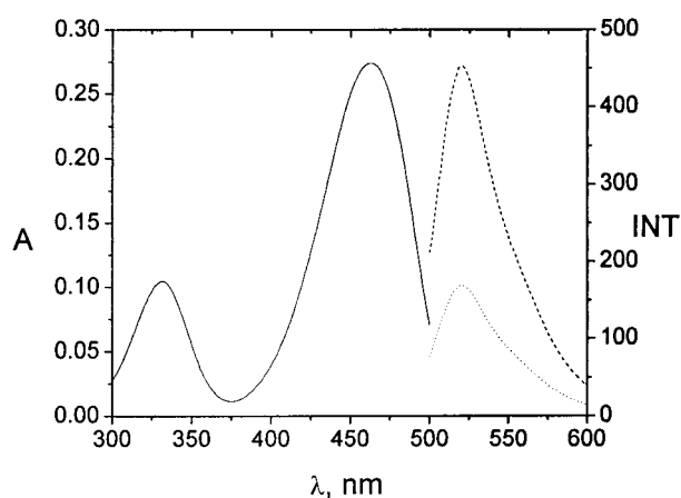
FIGURE 1 Absorption (—) spectrum and emission spectra of DPPN in methanol. The upper emission spectrum (---) was recorded with excitation at 470 nm, and the lower spectrum (---) with excitation at 335 nm. Spectra were measured at ambient temperature.
